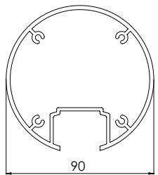
Monopole (round) 90
